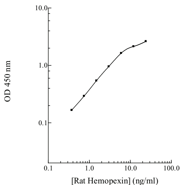
Rat Hemopexin Standard Curve
